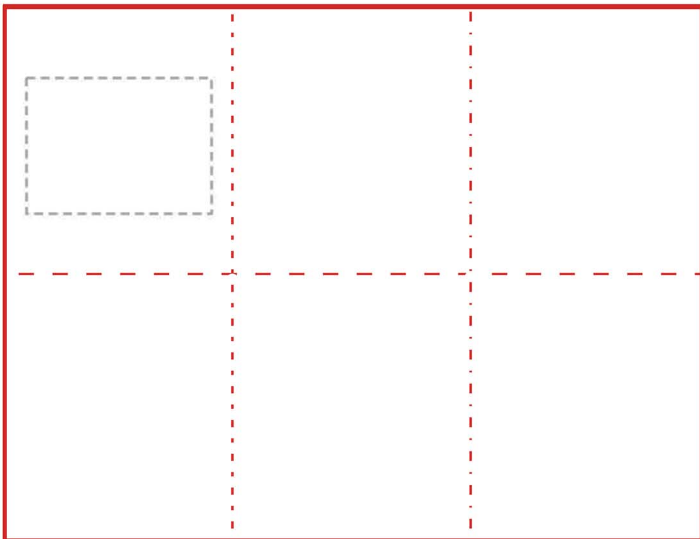
Rectangle
