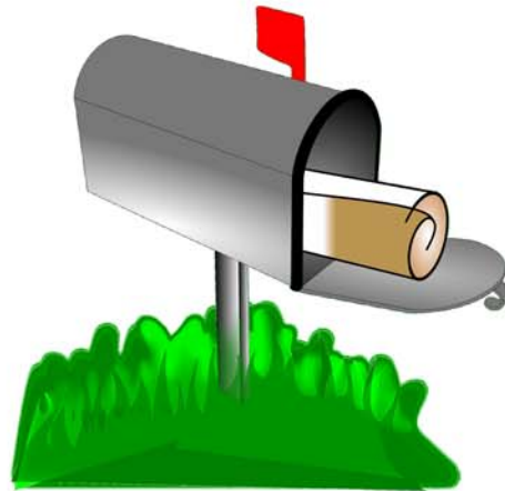
mail
